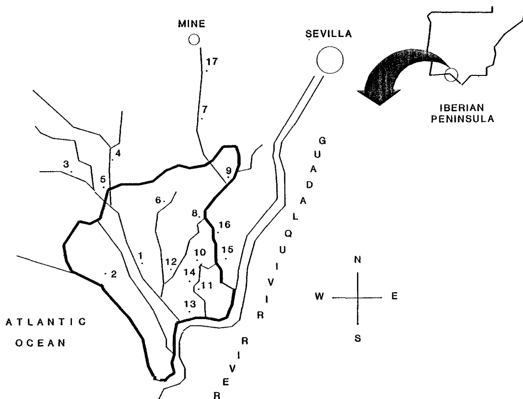
Fig. 1. Study area and sampling locations. Gross line is the limit of the park.
